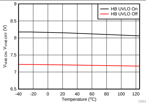
图 14. VHB-VHS UVLO Thresholds vs Temperature
