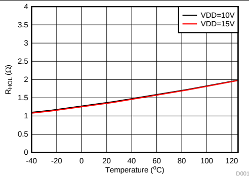
图 20. HO Output Pull-Down Resistance vs Temperature
