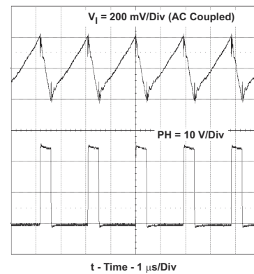
Figure 8-5. Input Voltage Ripple and PH Node, I_O = 5\text{ A} .
