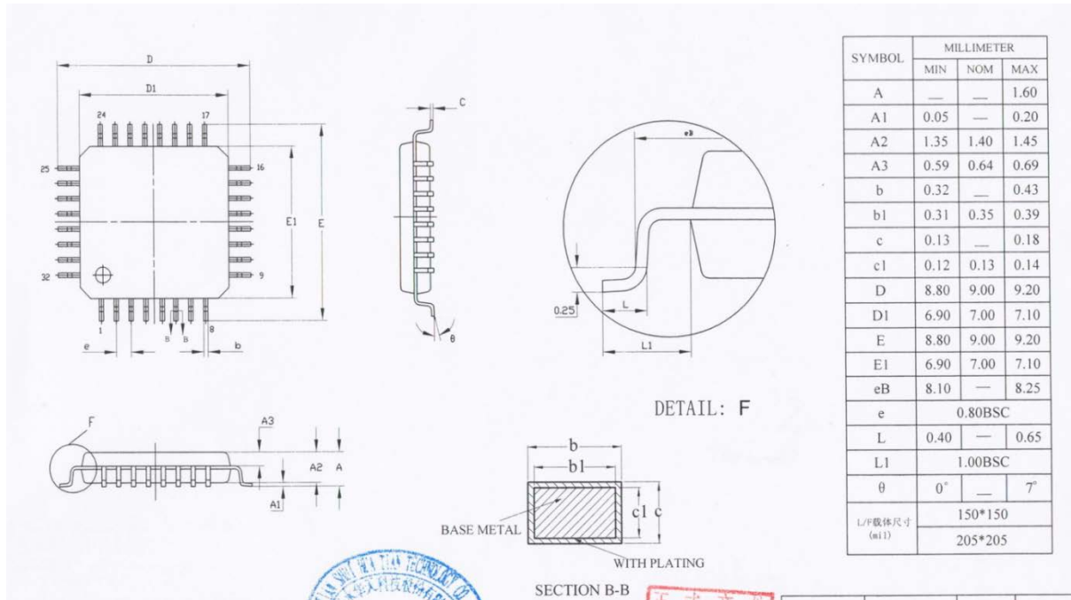
LQFP32
