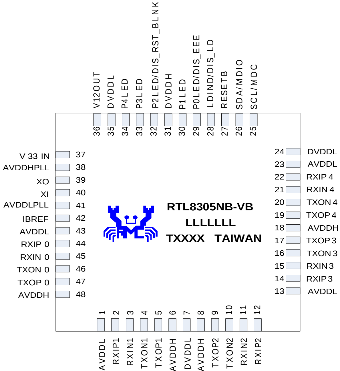
Figure 2. Pin Assignments
