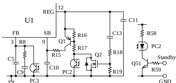
Figure 8-19. Standby mode change circuit
