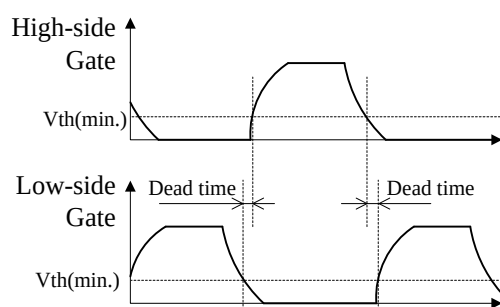
Figure 9-2. Dead Time Confirmation
