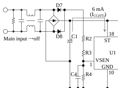
Figure 8-30. Input capacitor discharge
