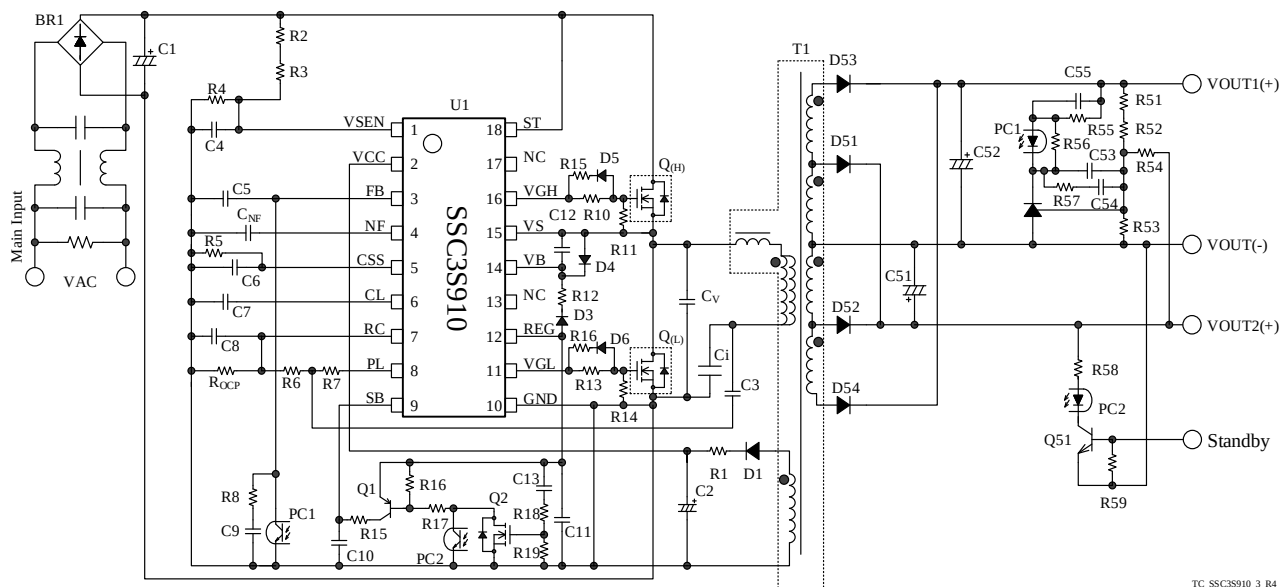
Figure 5-1. Typical application circuit
