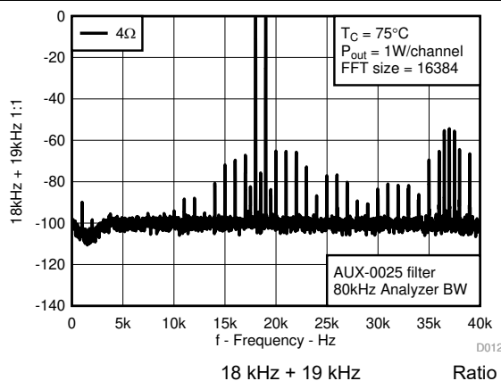
图 6-12. CCIF Intermodulation, AD-mode
