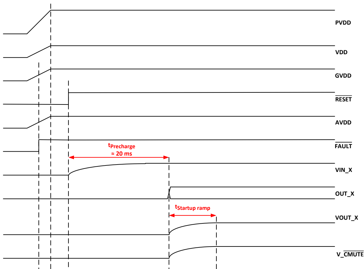
图 8-21. Startup Timing
