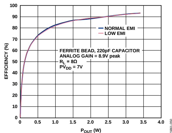
Figure 52. Efficiency vs. P_{OUT} , with Ferrite Bead, Analog Gain = 8.9 V peak, R_L = 8\ \Omega , PV_{DD} = 7\ V
