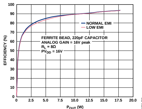
Figure 54. Efficiency vs. P_{OUT} , with Ferrite Bead, Analog Gain = 16 V peak, R_L = 8\ \Omega , PV_{DD} = 16\ V
