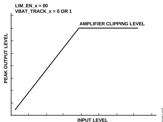
Figure 77. Limiter Example (LIM_EN_x = 00, VBAT_TRACK_x = 0 or 1)
