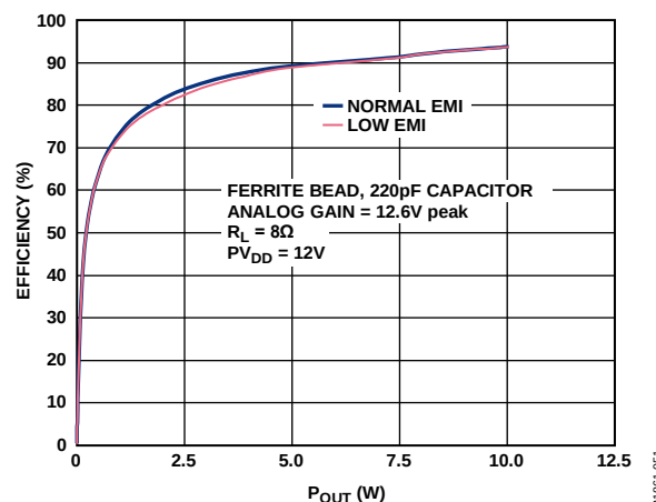
Figure 53. Efficiency vs. P_{OUT} , with Ferrite Bead, Analog Gain = 12.6 V peak, R_L = 8\ \Omega , PV_{DD} = 12\ V
