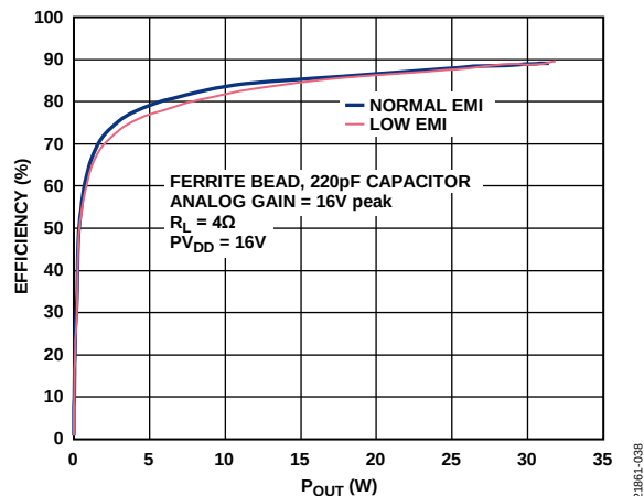
Figure 40. Efficiency vs. P_{OUT} with Ferrite Bead, Analog Gain = 16 V peak, R_L = 4\Omega , PV_{DD} = 16V
