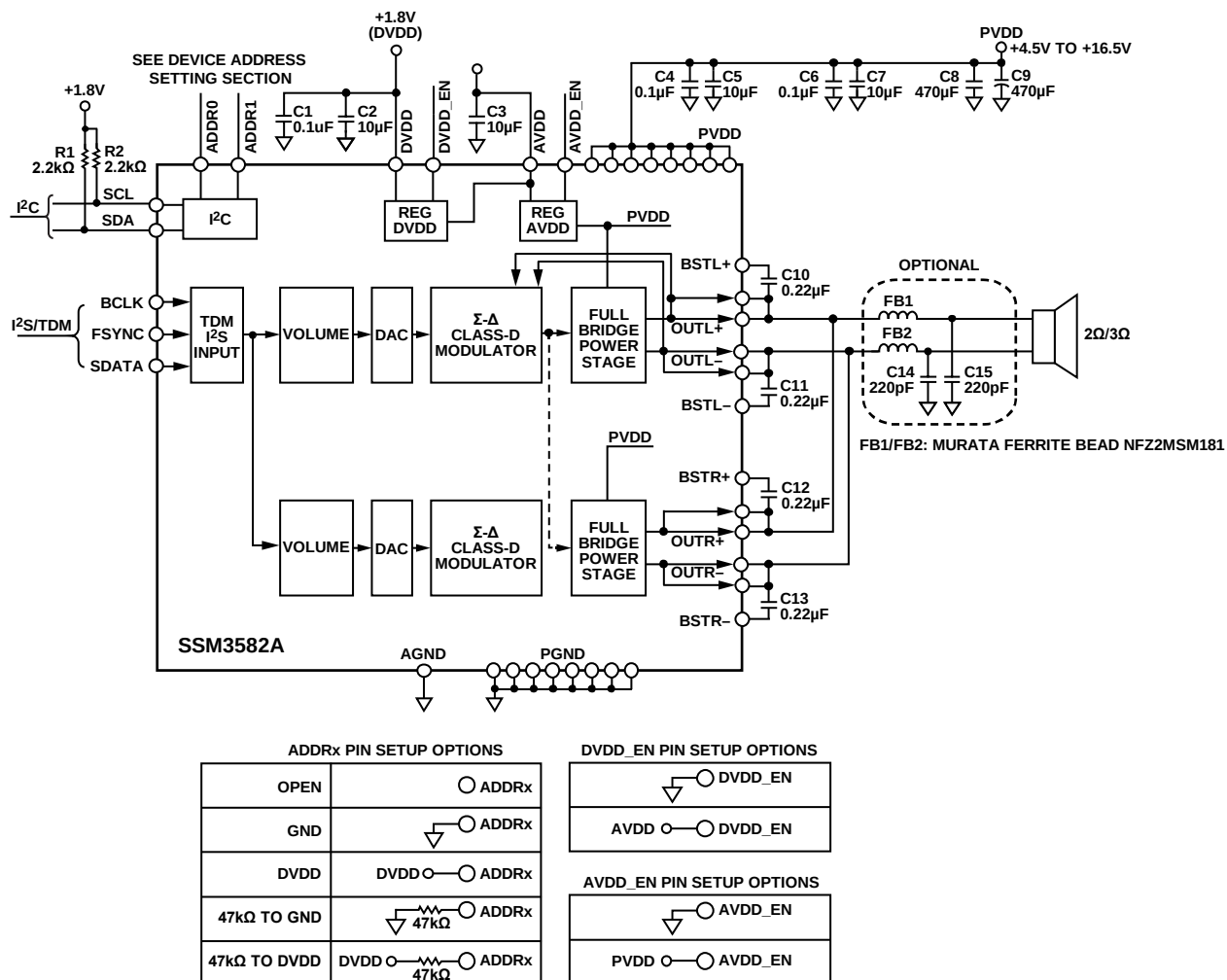
Figure 87. Typical Application Circuit for Mono Output
