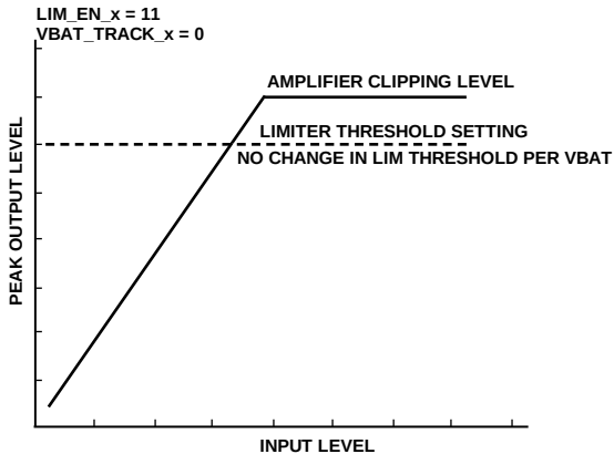
Figure 80. Limiter Example (LIM_EN_x = 11, VBAT_TRACK_x = 0)
