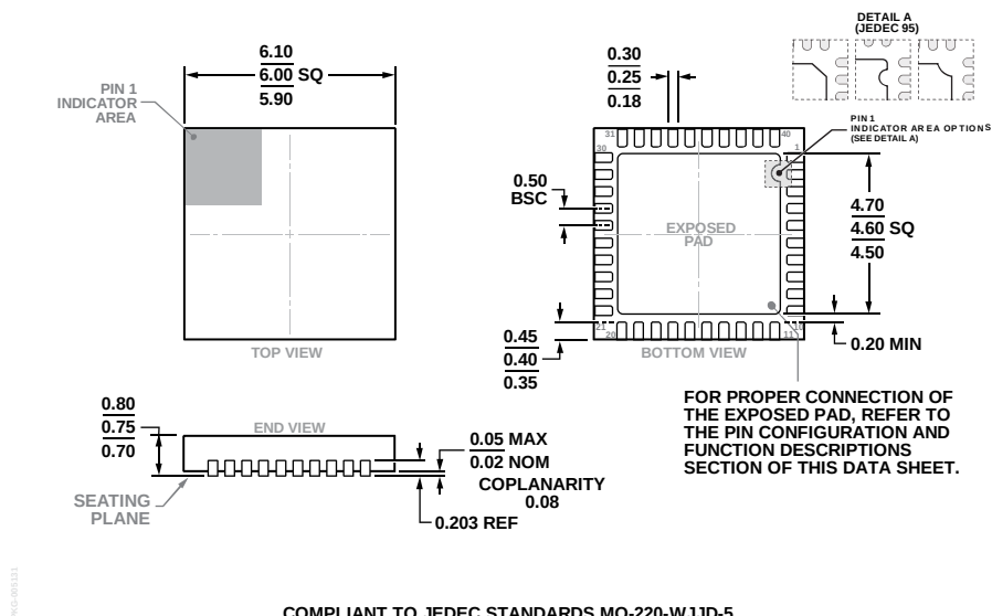
Figure 88. 40-Lead Lead Frame Chip Scale Package [LFCSP] 6 mm × 6 mm Body and 0.75 mm Package Height (CP-40-7)
