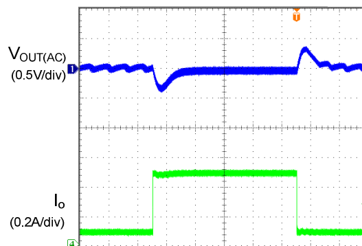
Load Transient
