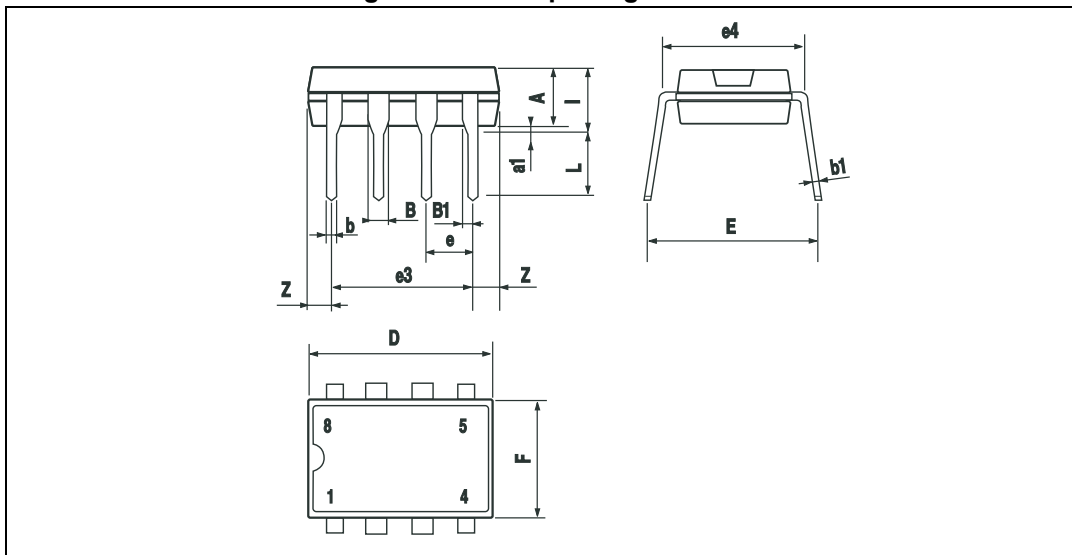
Figure 15. DIP-8 package outline
