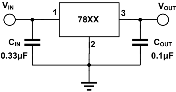
(1) Conventional Circuit
