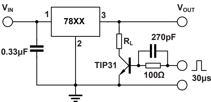
Figure 9-6. Load Regulation
