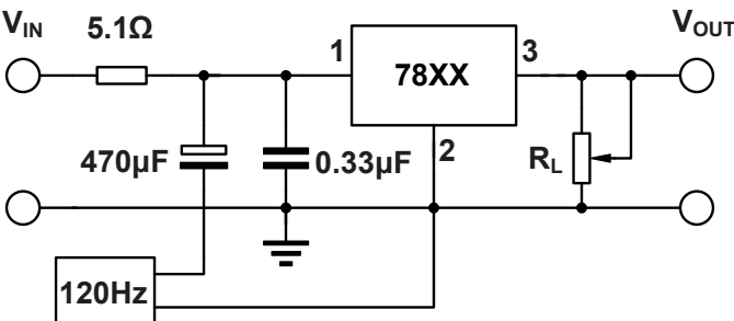
Figure 9-7. Ripple Rejection
