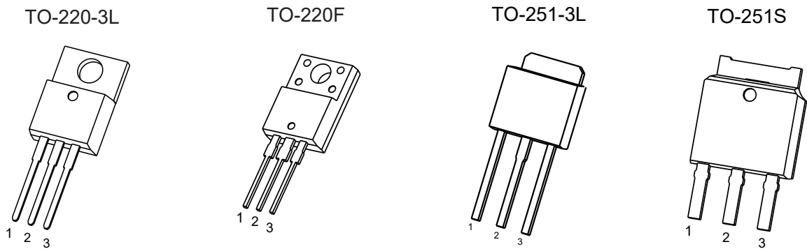
Figure 6-1. CJ78 Series Package Top View
