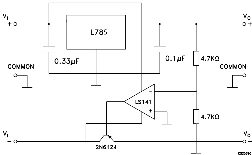
Figure 24. Tracking voltage regulator
