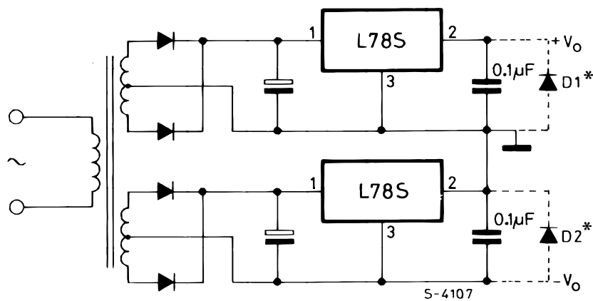
Figure 25. Positive and negative regulator
