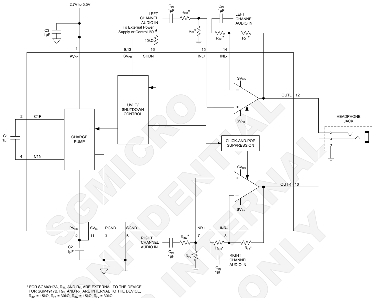
Figure 2. Typical Differential Input Application Circuit
