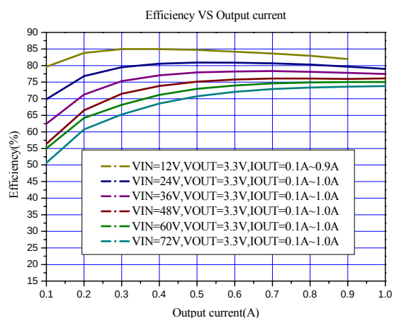
Figure15. VIN=8V~80V, VOUT=3.3V
