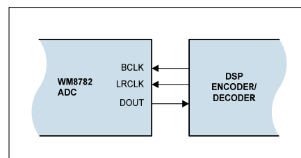
Figure 7 Slave Mode
