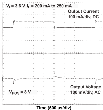
图 8-41. Load Transient Response
