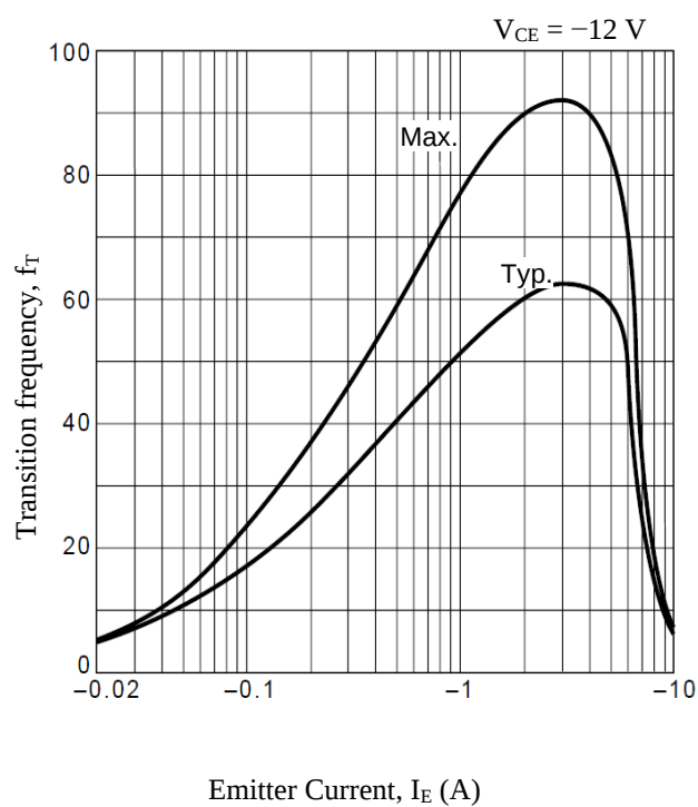
Figure 8. Transition Frequency vs. Emitter Current
