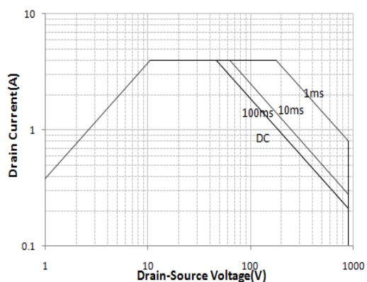
Maximum safe operating area (JCS4N90VA/RA/CA/BA)
