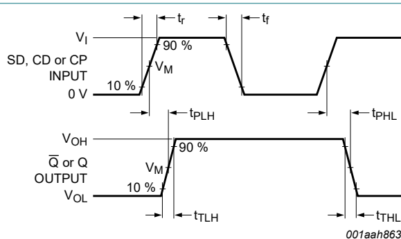
Fig. 4. Waveforms showing rise, fall, and transition times, and propagation delays
